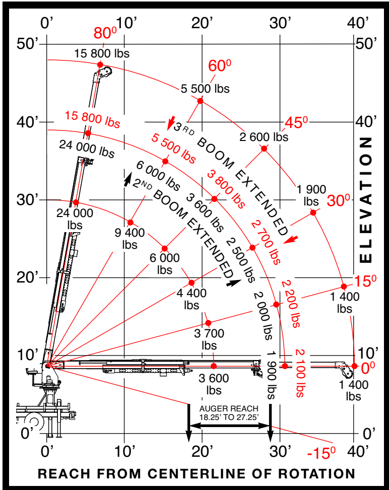
HERCULES 20K50 Typical load chart for 33 000 lb GVW trucks Actual load chart to be determined based on final truck configuration, outrigger options and boom options
